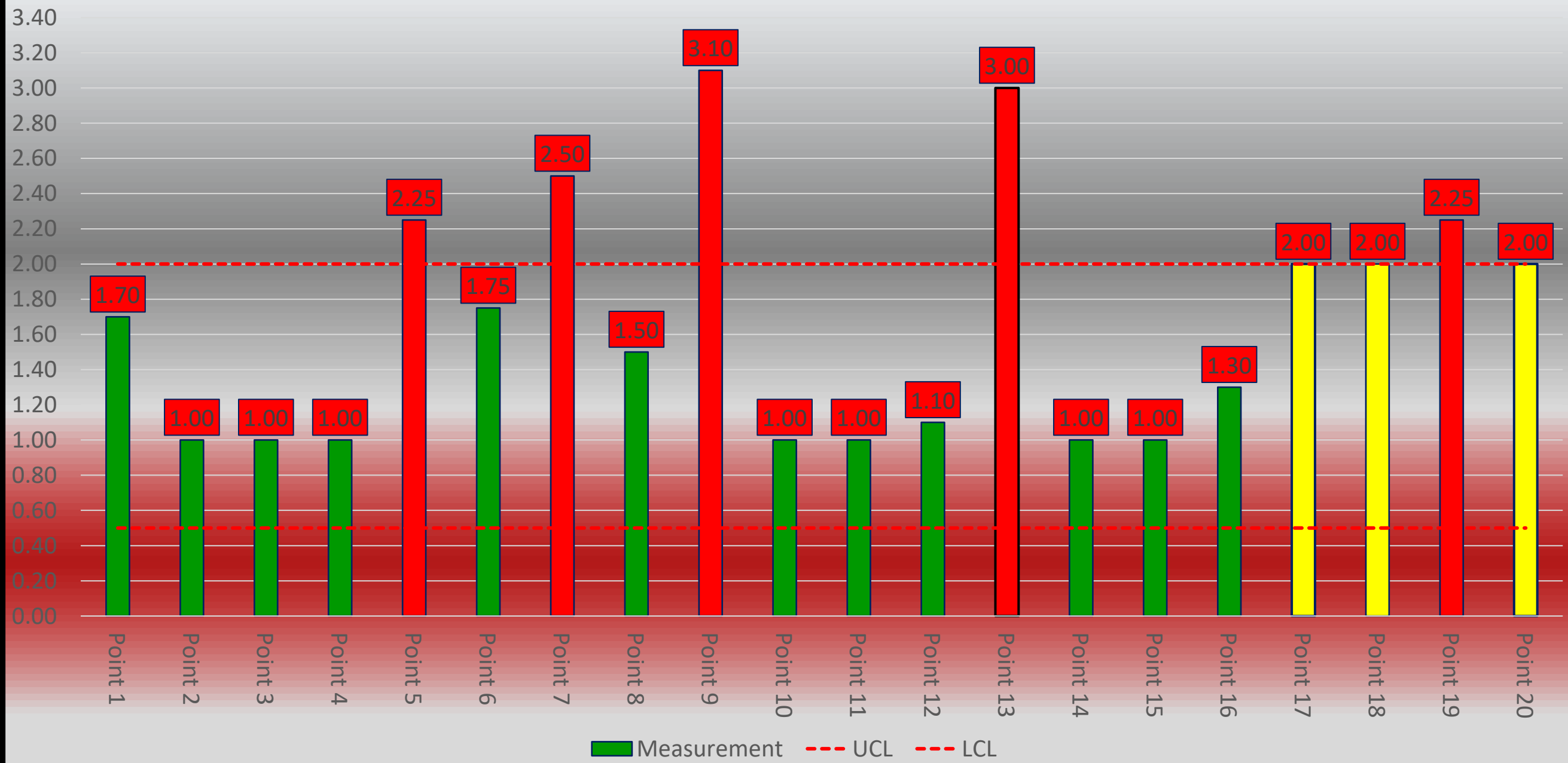
Gap Measurement Data B Pillar AC LH With Laminated Fabric
